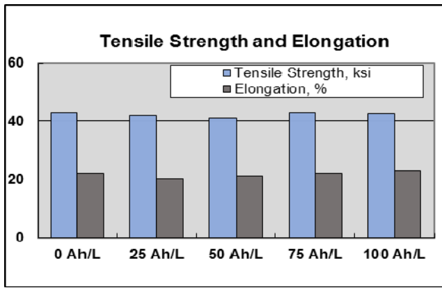
Figure 18. Tensile Strength and Elongation at different stages of the bath life.
