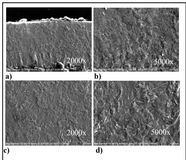
Figure 23. SEM. a) and b) Cross Section pictures of the Surface around 4x3 via; b) and c) Cross Section pictures of copper plated inside 4x3 via. Panel Plated at 20 ASF.
