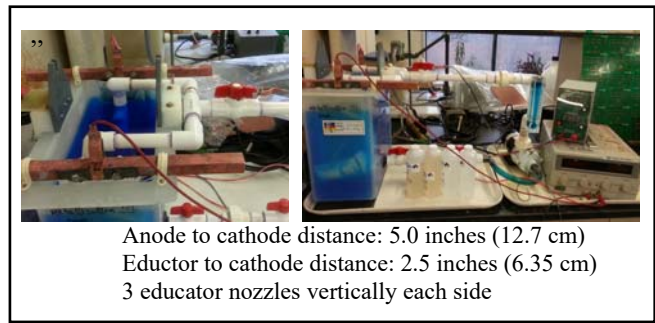
Figure 1. 12 liters plating cell.
