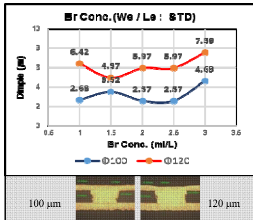
Figure 11. Via Dimple as a function of Brightener concentration in the bath.
