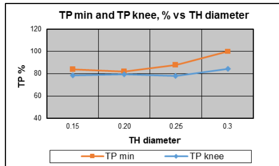
Figure 8. TP min and TP knee for various TH sizes.
