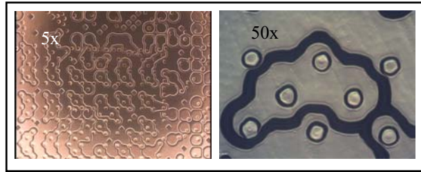
Figure 20. Surface of a panel plated in VF-TH 200.
