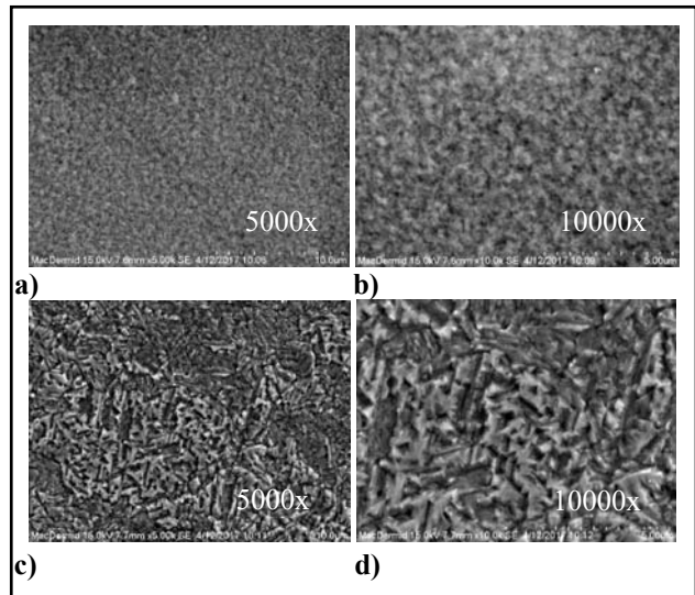
Figure 24. SEM. a) and b) Panel surface, top view; c) and d) Panel Surface, top view after Etching. Plating at 20 ASF.
