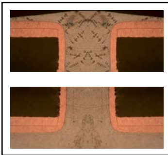
Figure 19. Cross section of 0.25 mm TH after 6x Solder Shock; plating at 20 ASF.
