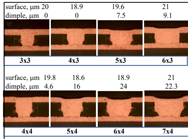
Figure 4. Cross sections of various diameter vias sizes, 3 and 4 mils deep (75 and 100 microns deep).
