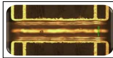
Figure 21. Cross section of a TH, diameter 0.25 mm, 0.8 mm thick panel.
