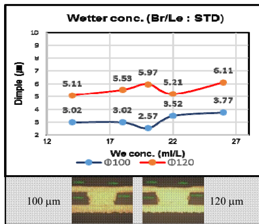
Figure 10. Via Dimple as a function of Wetter concentration in the bath.
