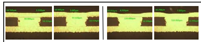
Figure 5. Cross sections of 50 microns deep vias, diameters: 100 and 120 microns.
