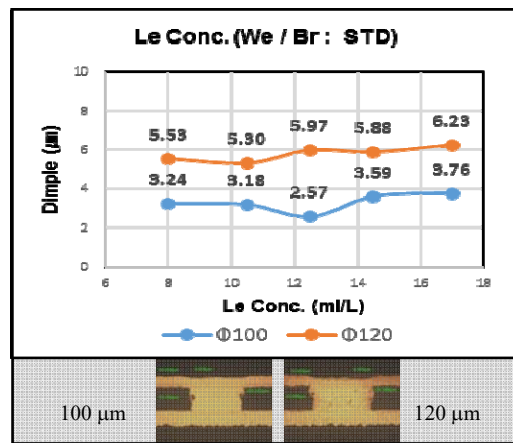
Figure 12. Via Dimple as a function of Leveler concentration in the bath.
