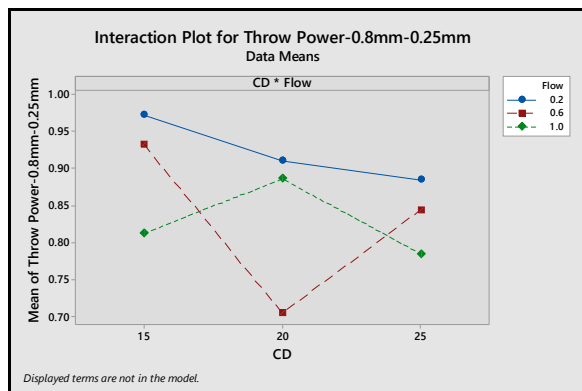
Figure 15. Throwing power, TP min of 0.25mm hole, 0.8 mm board, interaction plot.
