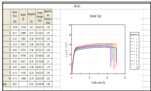
Figure 17. Tensile Stress and Elongation measurements, bath age 100 Ah/L
