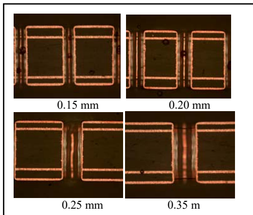
Figure 7. Cross sections of plated through holes; hole diameters 0.15, 0.20, 25, and 0.30 mm.
