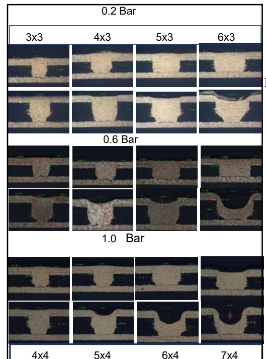
Figure 13. Cross sections of vias plated at solution flows: 0.2, 0.6, and 1.0 Bar.
