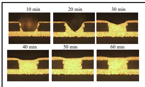
Figure 9. Stages of via fill process. BMV 100 x 60 microns; target Cu thickness 15 microns.
