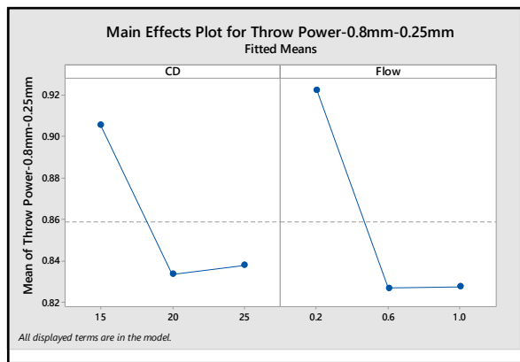
Figure 14. TP min for a 0.25 mm diameter hole in 0.8 mm board as a function of CD and solution flow.
