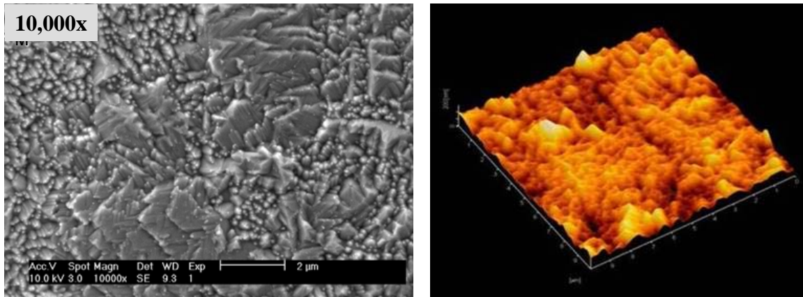
Figure 8: Structure of Peroxide Etched Copper by SEM and AFM
