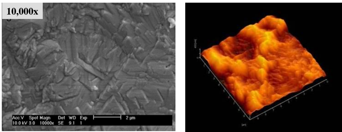
Figure 9: Structure of Persulfate Based Etched Copper by SEM and AFM
