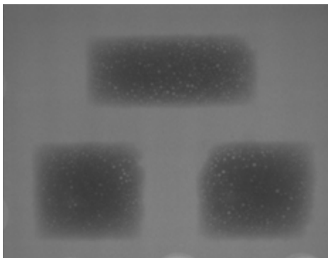
Figure 1 X-ray View of Microvoiding in Soldered Pads
