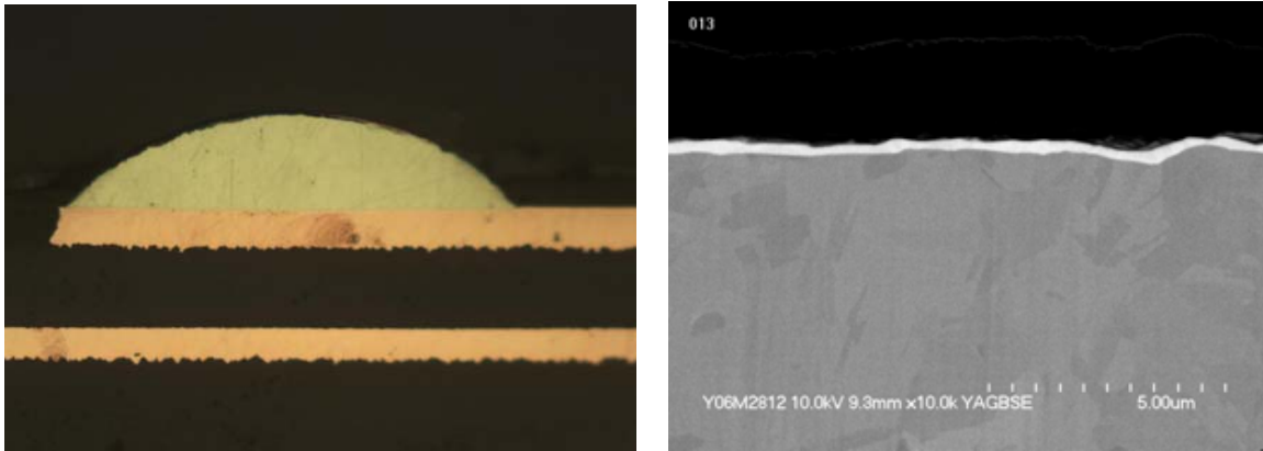
Figure 17: Microvoid-free and Cave-free Samples Produced With New Best Practice Conditions
