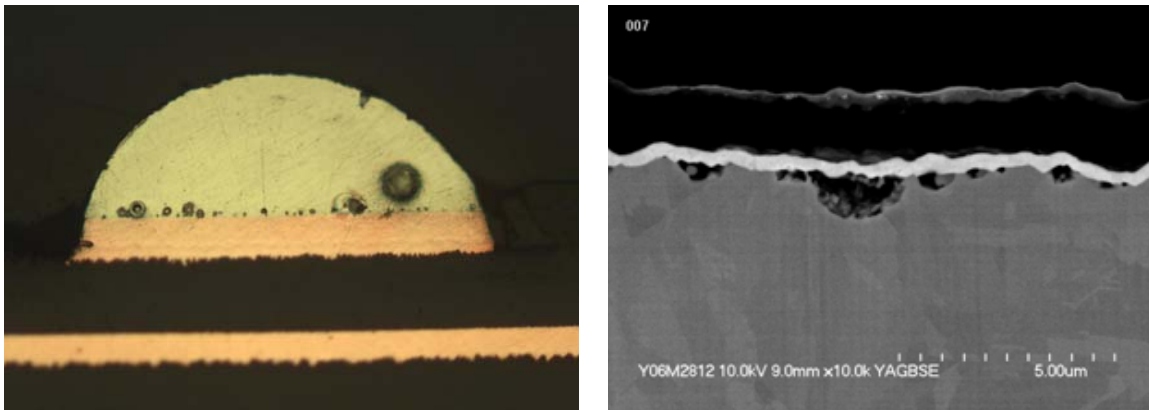
Figure 16: Microvoids and Caves (FIB analysis) Produced Under Old Operating Conditions
