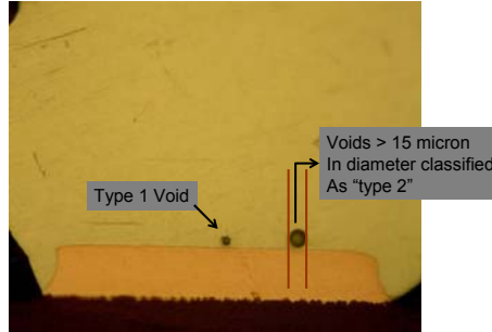
Figure 18: Illustration of Type 1 and Type 2 Microvoids
