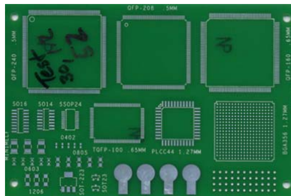
Figure 4: Standard Test Vehicle with BGA Feature
